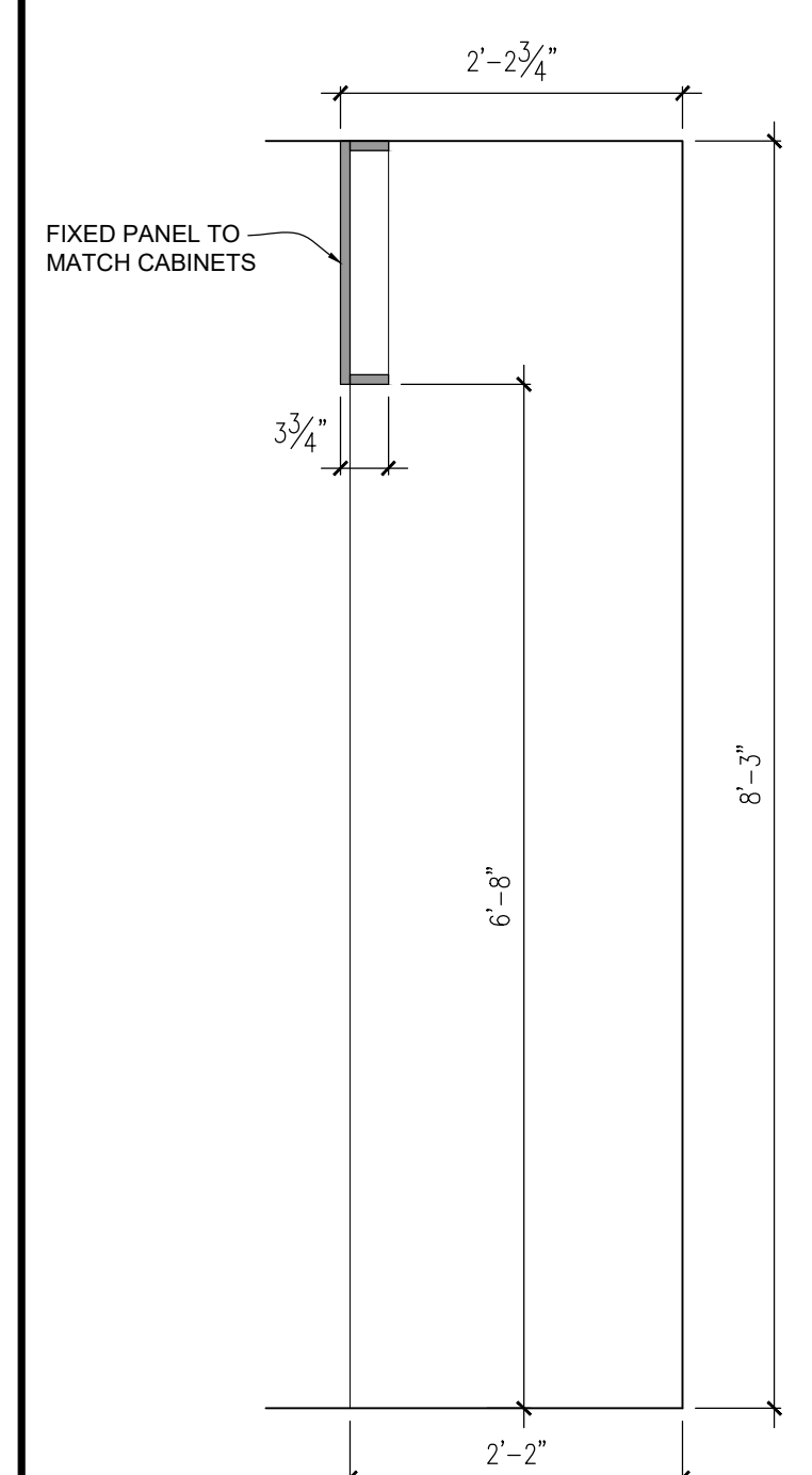
E SECTION
