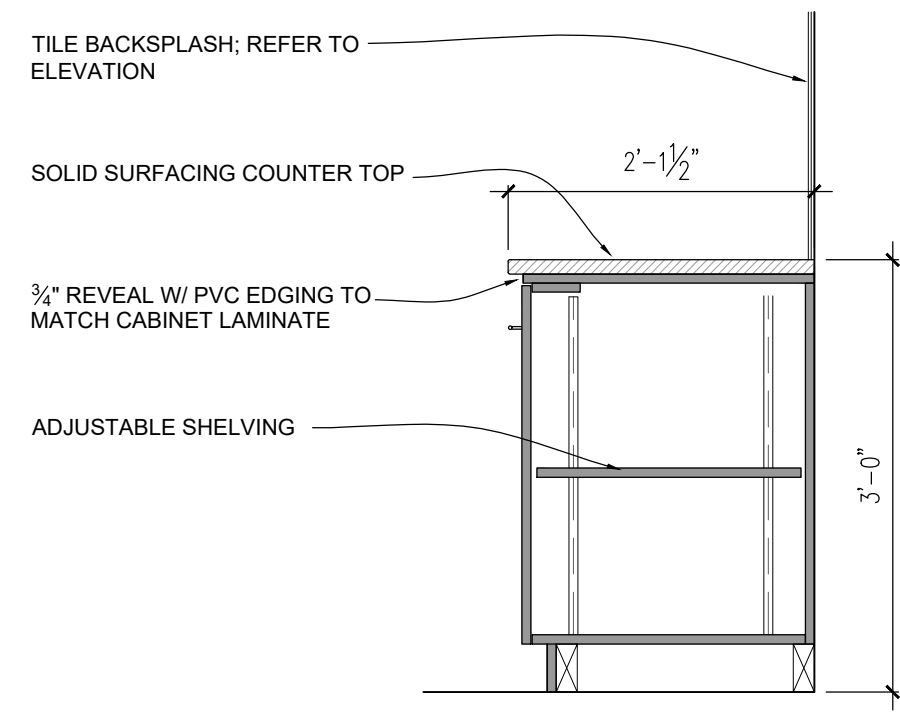
A SECTION
