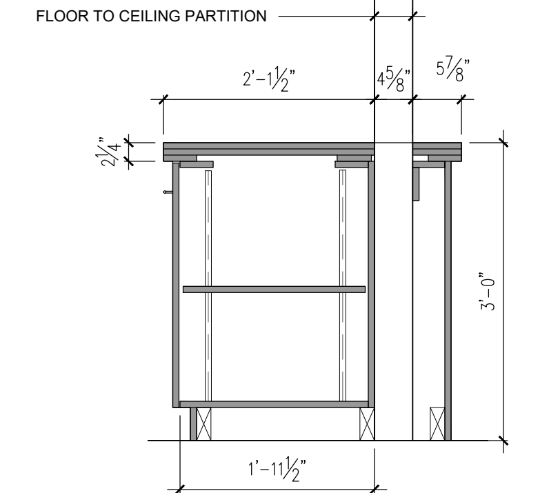
N SECTION
