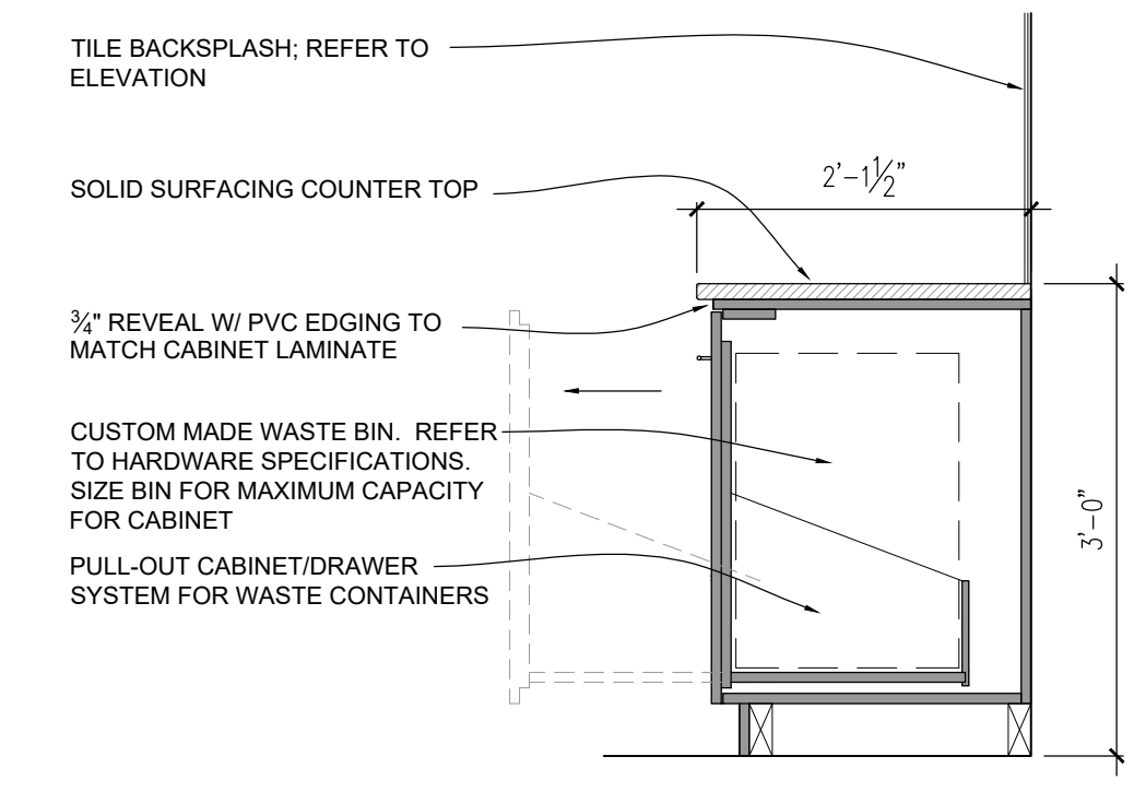
D SECTION
