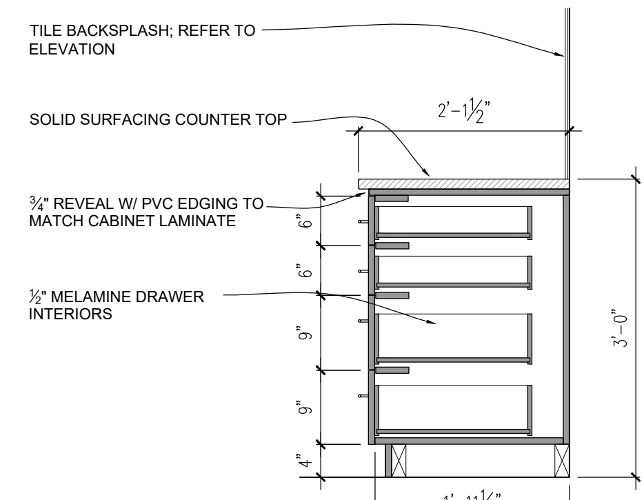
B SECTION
