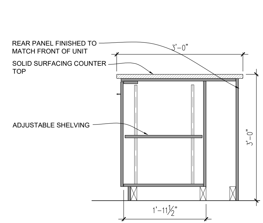
H SECTION
