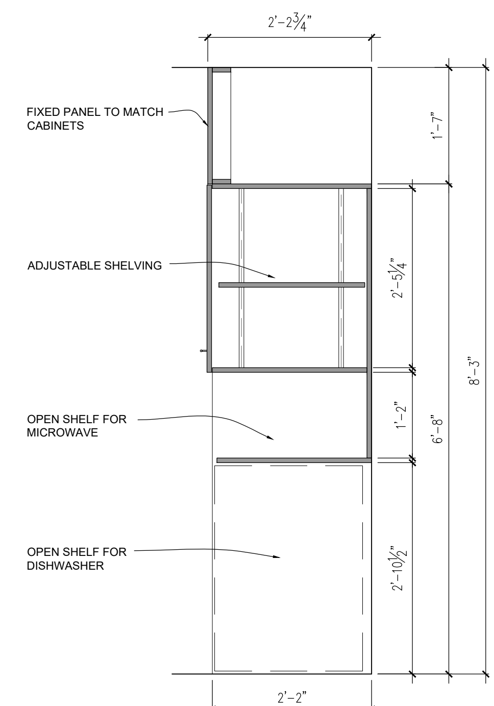
F SECTION
