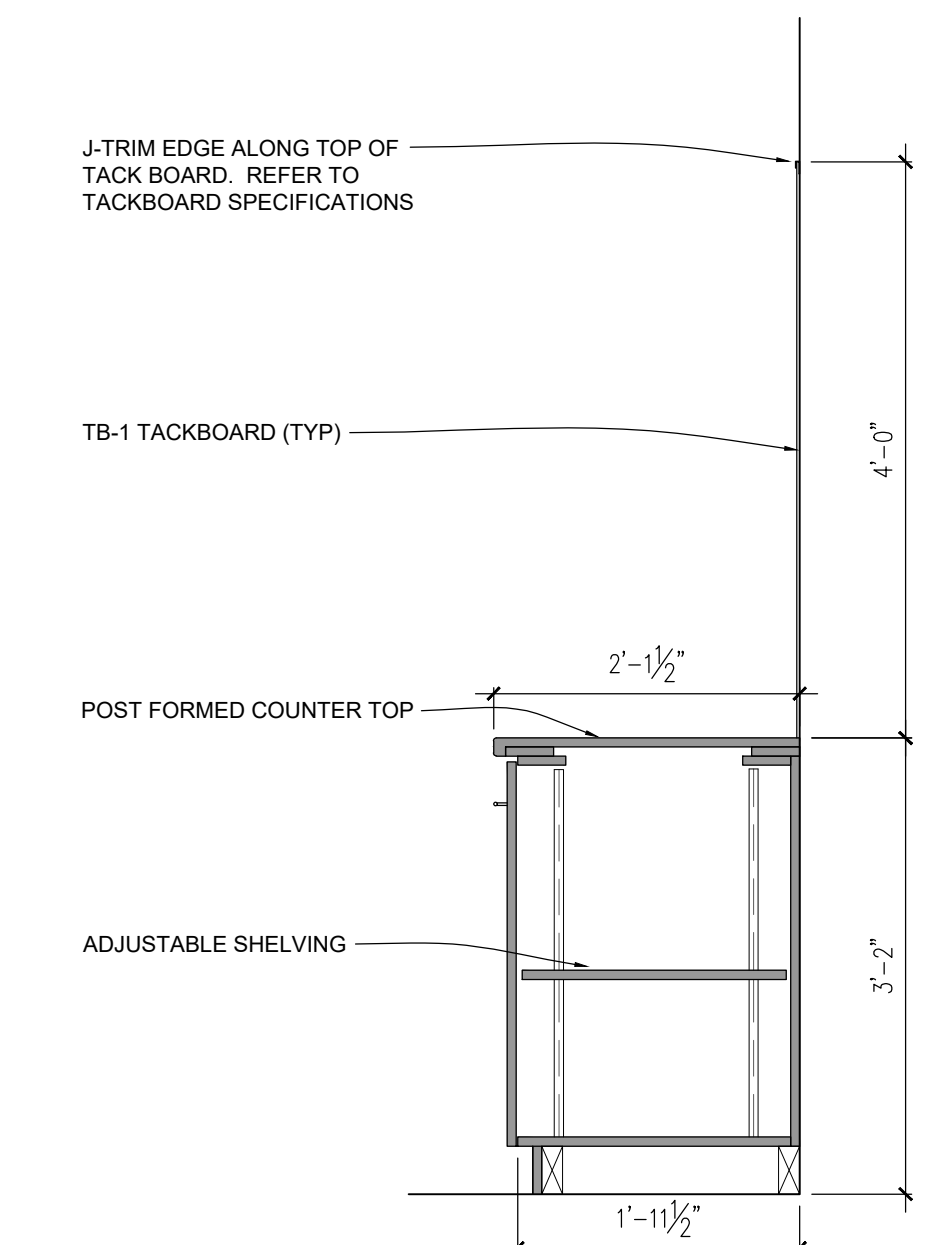
R SECTION
