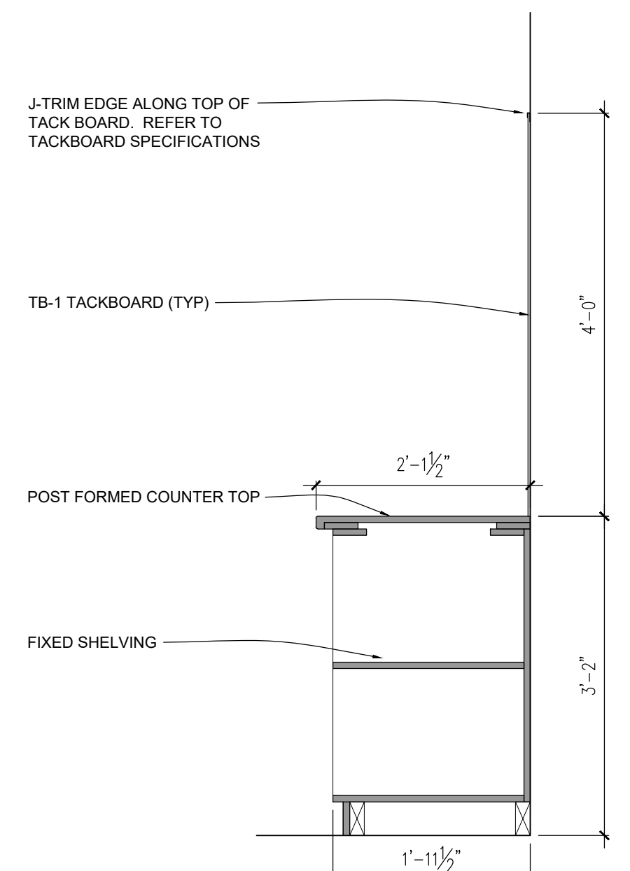
P SECTION
