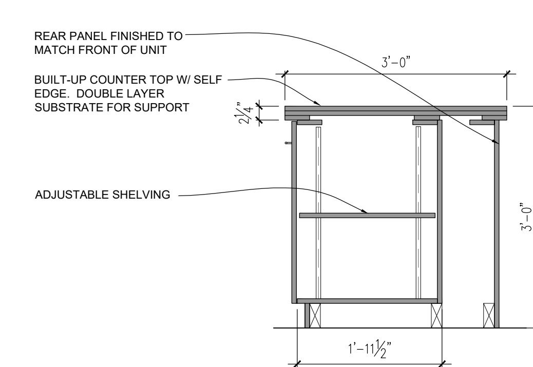
M SECTION
