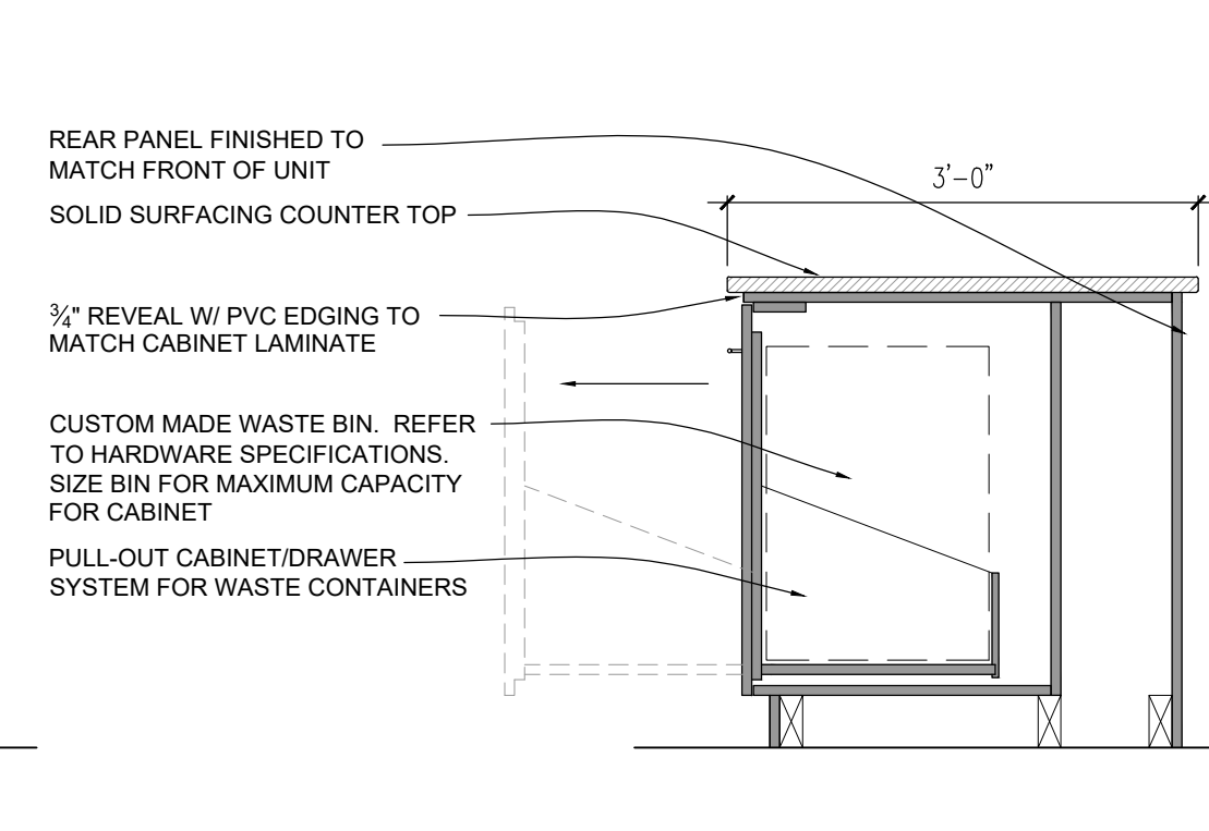
K SECTION
