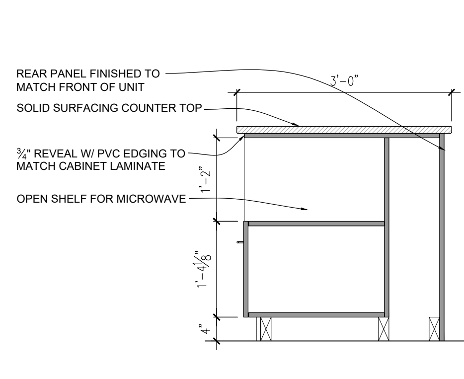
I SECTION
