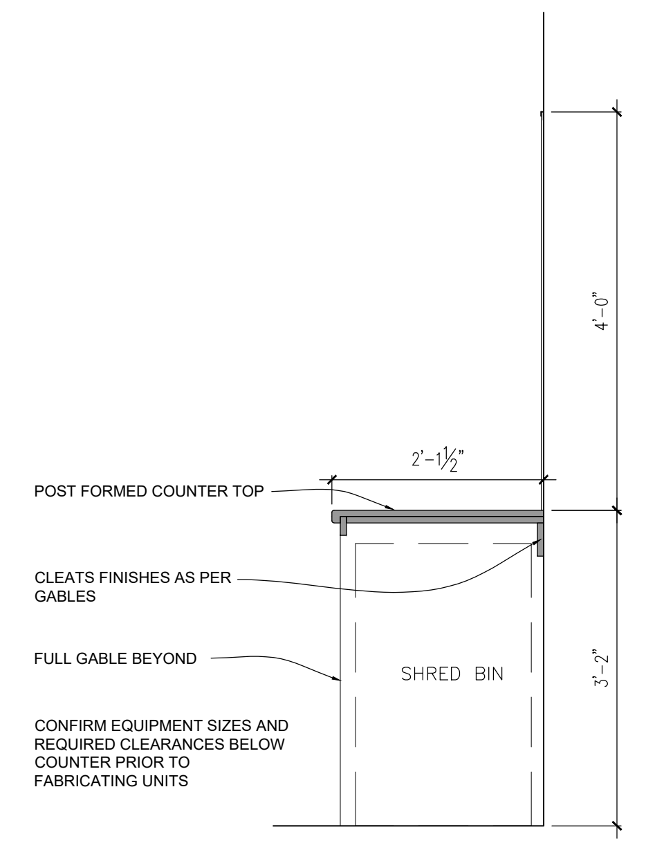
T SECTION
