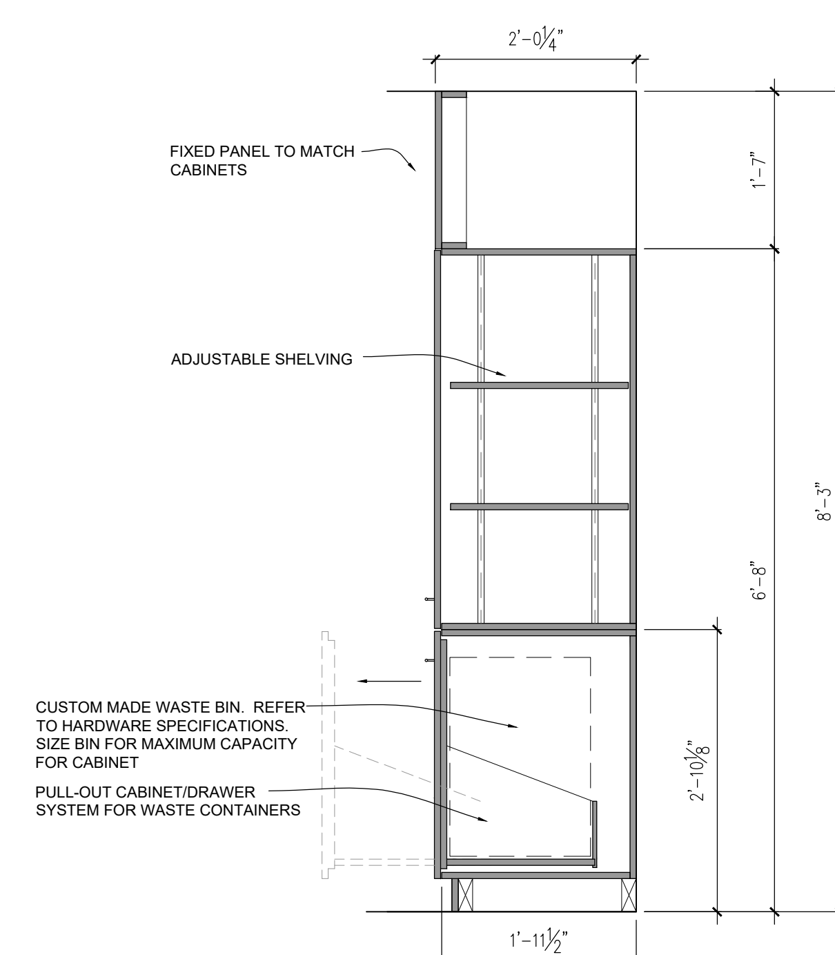
G SECTION
