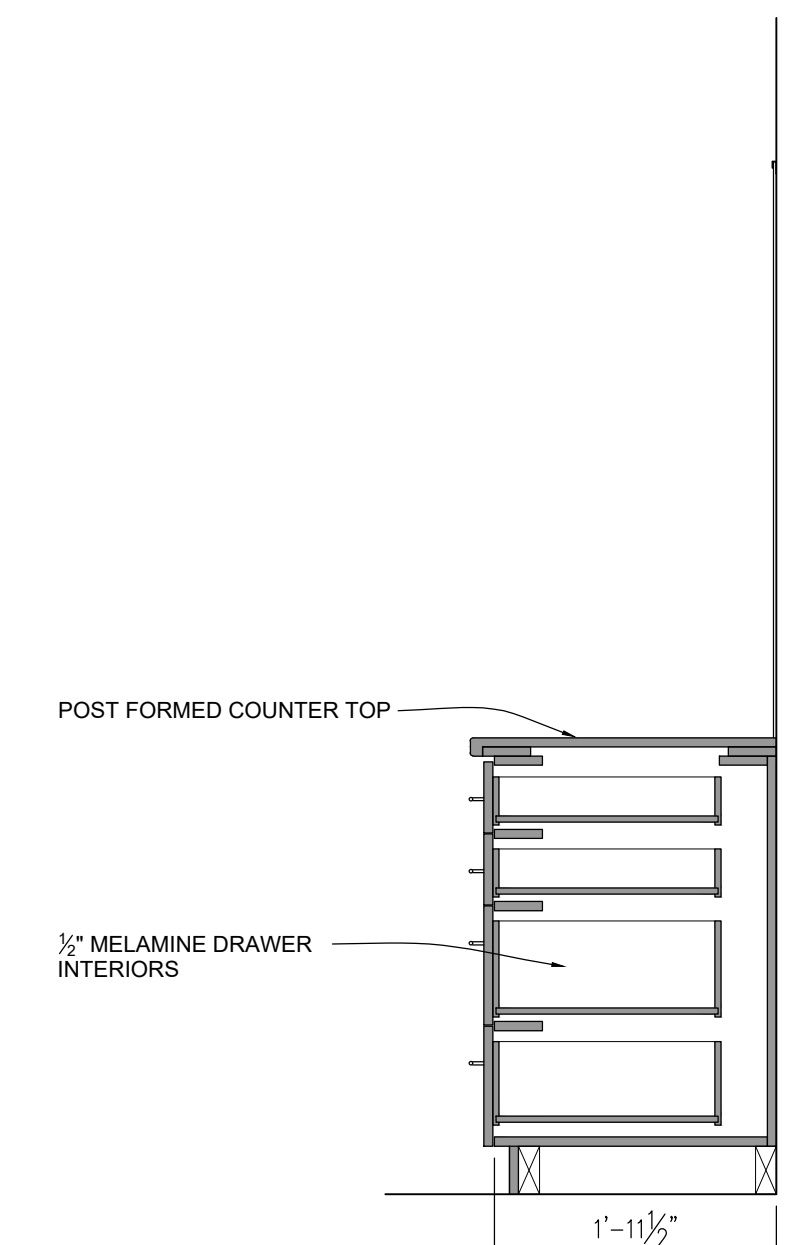
S SECTION
